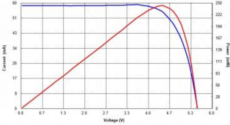
Current-Voltage Characteristics @1sun AM1.5 25°C
